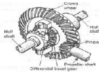
(ii) Typical three-dimensional view
