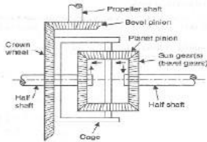
(i) Simple differential-simplified diagram
