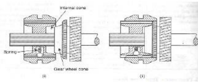
Synchromesh unit
