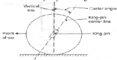
Caster angle (Positive)
